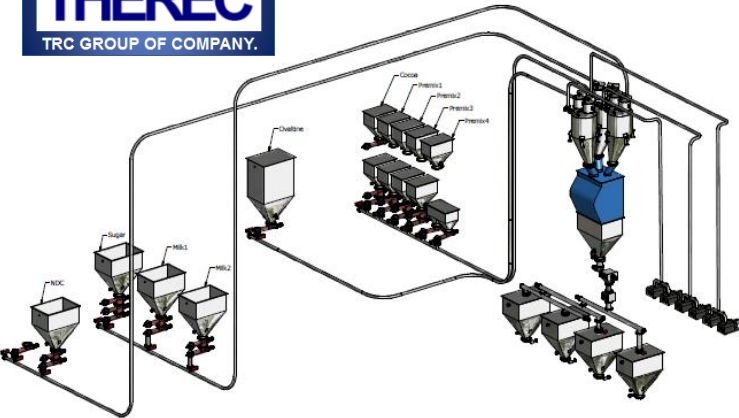
AB Food (Thailand) Co., Ltd. / Ovaltine Three in one raw material conveying system Sugar, Coco powder, Milk powder
