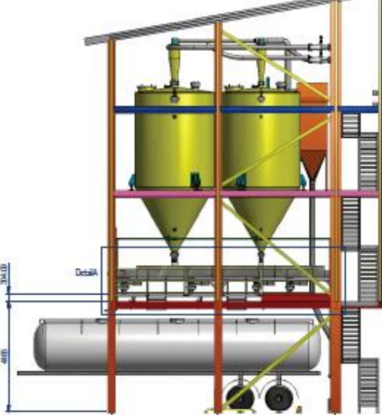
Thai Plastic (Public) Co., Ltd. / SCG Chemical PVC powder container loading system , from 100 tons storage silos to container Mobile (on truck) special design for inter plant movement
