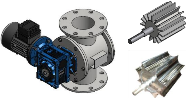
Thai Plastic Bag Co., Ltd./ Calcium carbonate powder weighting system by Dosing rotary valve
