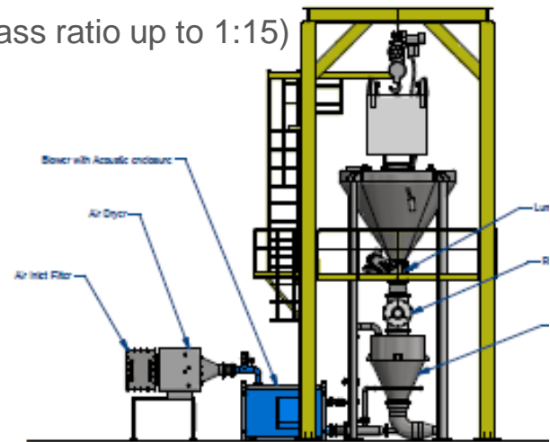
Mitr Phol Sugar Corp., Ltd. Sugar loading system from big bag unloading station to container loading station
