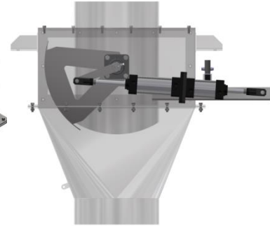
Thai Poly Ethylene Co., Ltd./ LLDPE Big bag filling station weighting system by Cut off valve
