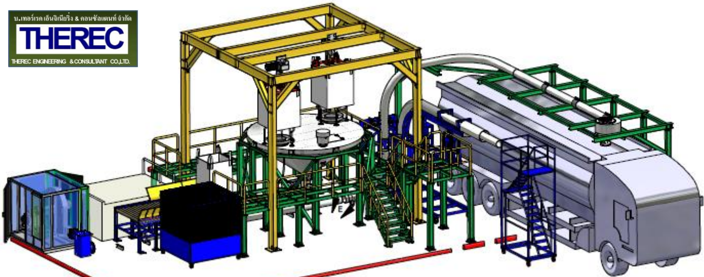
PTT Global Chemical (Public) Co., Ltd. / Poly ethylene Pellet Seal bulk loading systems , from big bag to container and bulk truck High pressure loading system (Roots blower / Air compressor)
