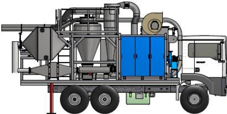
Thai Plastic (Public) Co., Ltd. / SCG Chemical PVC powder container loading system , from 100 tons storage silos to container Mobile (on truck) special design for inter plant movement
