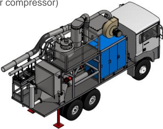
Thai Plastic (Public) Co., Ltd. / SCG Chemical PVC powder container loading system , from 100 tons storage silos to container Mobile (on truck) special design for inter plant movement
