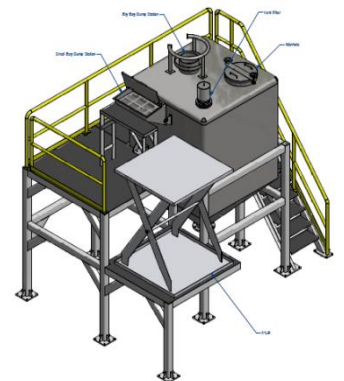
Big bag & Small bag dumping station With over head crane and X lifter
