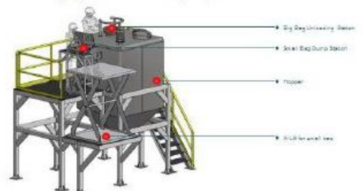
Big Bag Unloader with Small bag Dump Station
