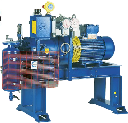
Rotary vane gas compressor
