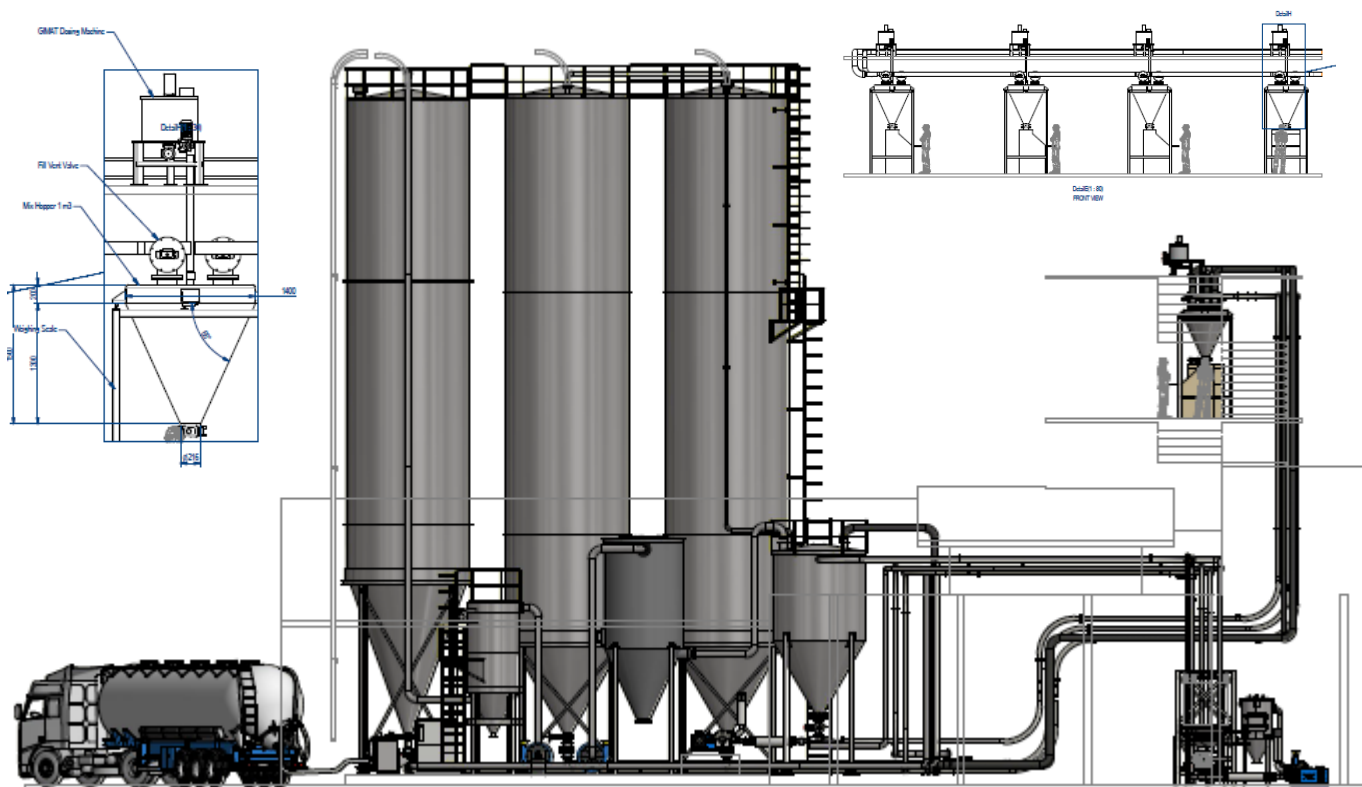
Silos Weighting system (PVC powder & Calcium Carbonate Powder ) Saha Aree , Twin Lion brand PVC pipe factory
